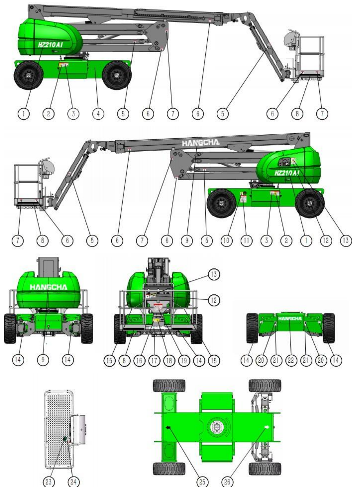
Figure7-1 adhesive signs
