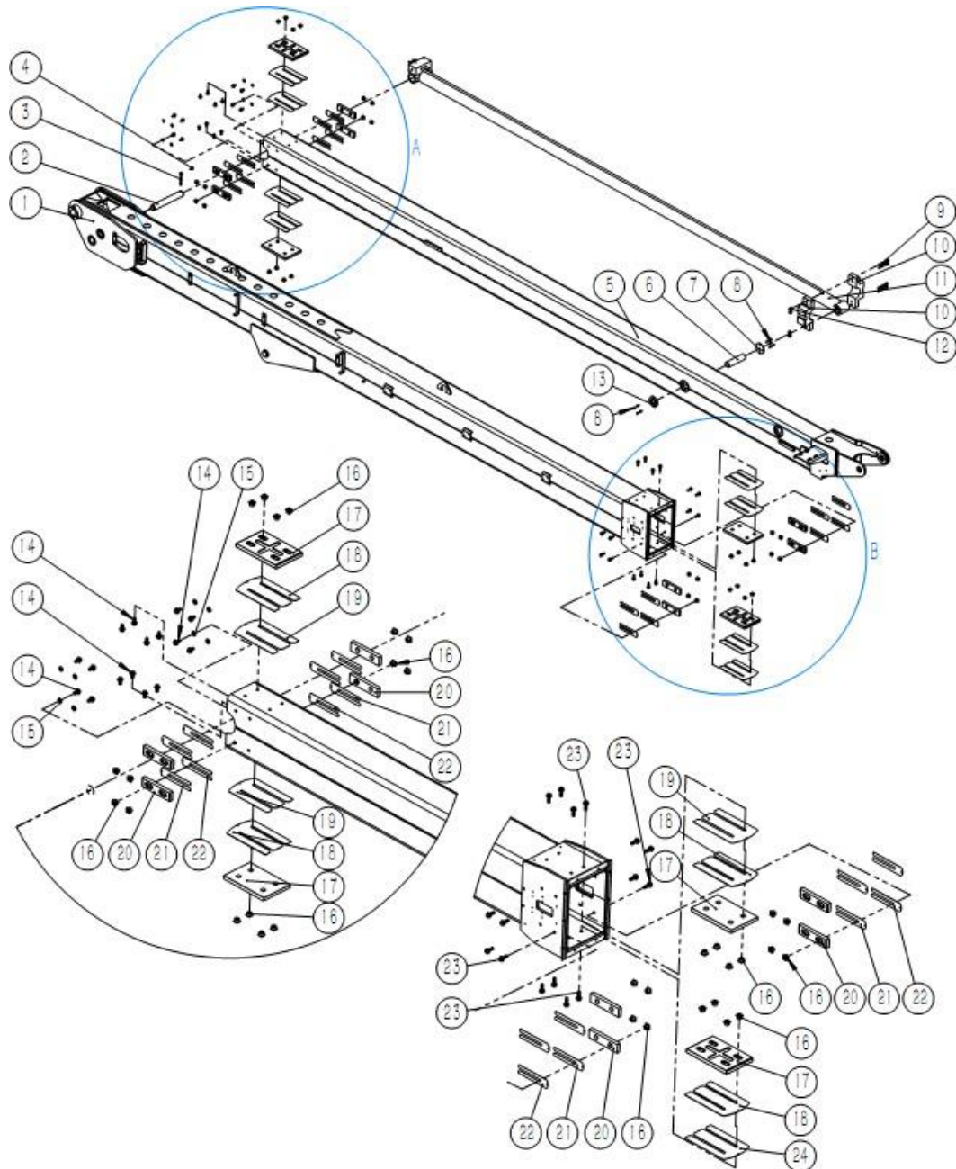
Figure 3-4 Upper secondary boom and telescopic boom assembly
