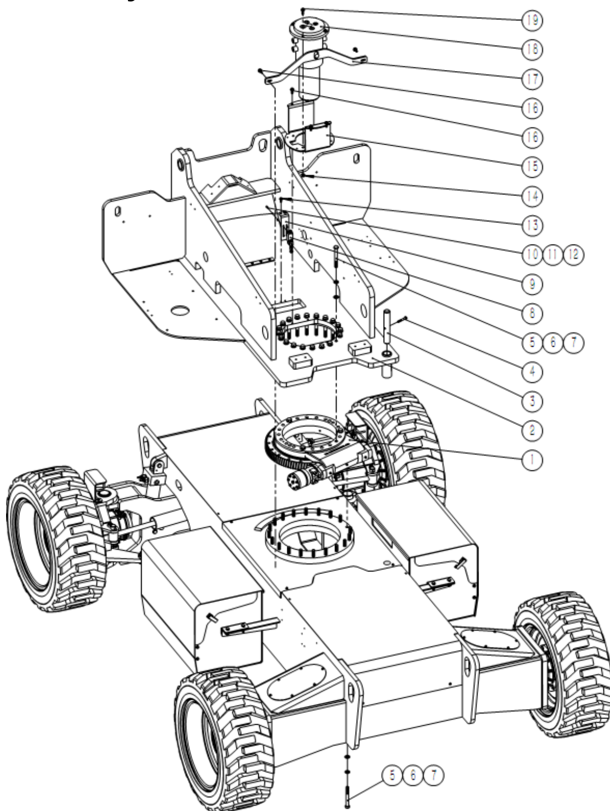
Figure2-1 Rotating frame and chassis a assembly
